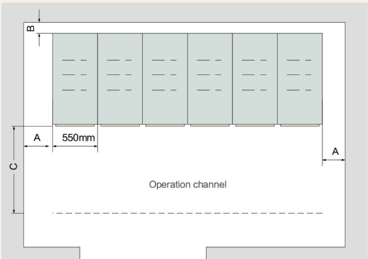
Distance between functional unit and wall
