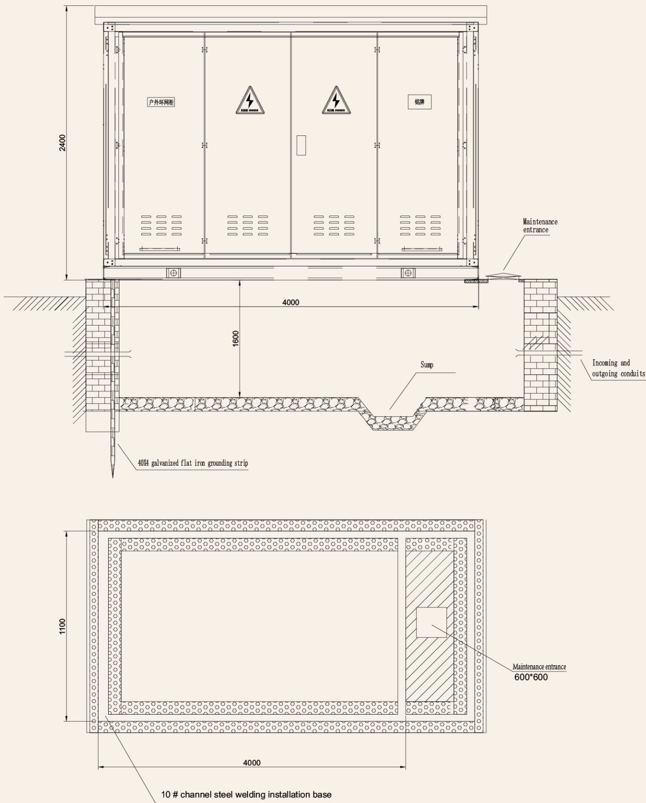
Basic diagram of outdoor box
