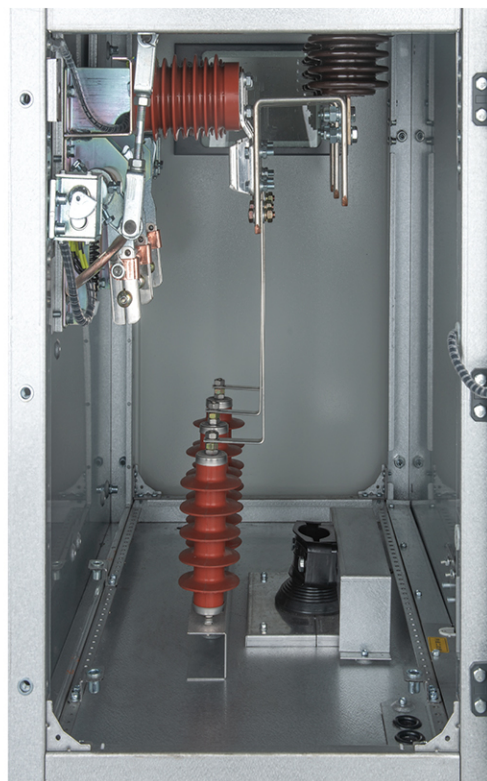
Cable Compartment
